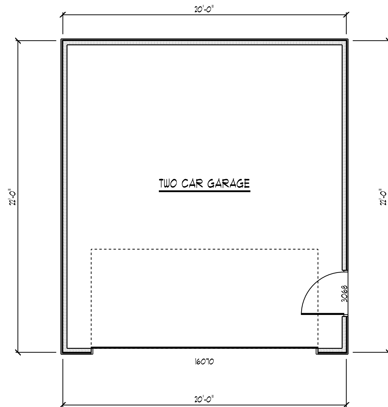
DETACHED GARAGE PLAN 1/4"=1'-0"
