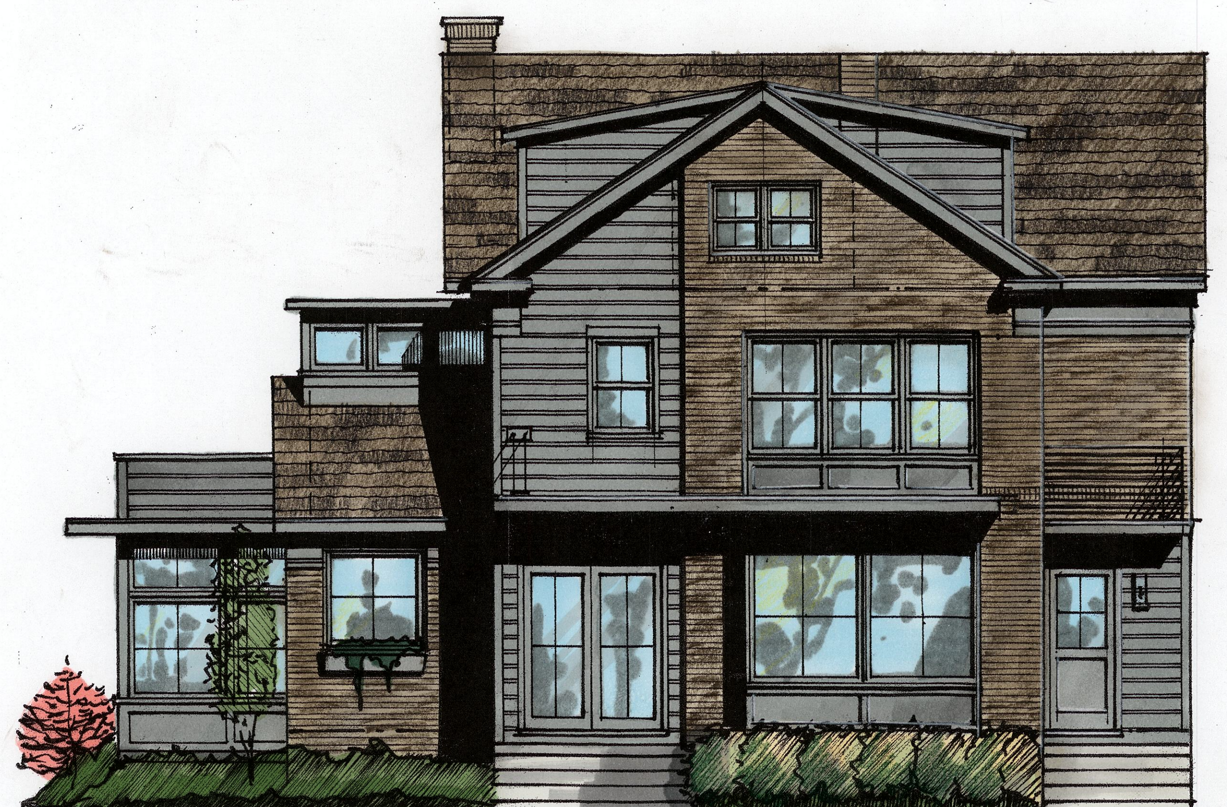
North Elevation 1/4" = 1' - 0"
